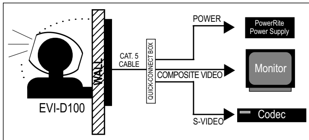
Figure 1 – EZCamera cable system with a quick-connect single gang wallplate/quick-connect box.
