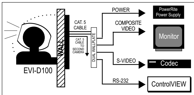
Figure 2 – EZCamera cable system with a quick-connect dual gang wallplate.
